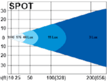
GXL™ LED Light Beam Dimensions
